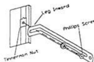
Figure 2a "L" Bracket Installation
