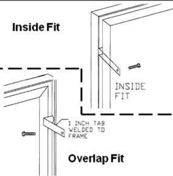
Figure 2a "L" Bracket Installation
